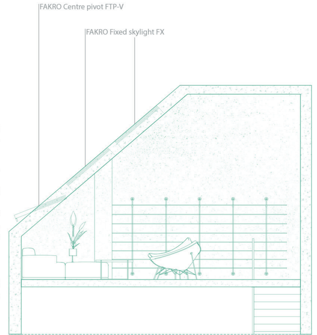
section / scale - 1:50 position of the windows
